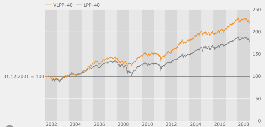
Fundo VLPP-40 vs LPP-40 01.01.02-31.12.18
