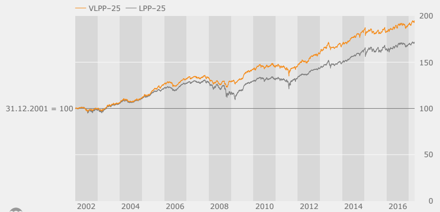
Fundo VLPP-25 vs LPP-25 01.01.02–31.03.17
