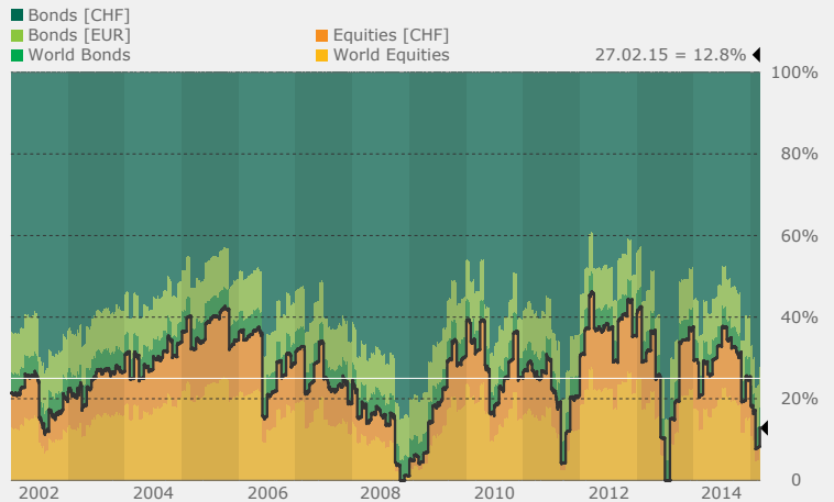
Fundo VLPP-25 Asset Class Weightings 01.01.02–27.02.15
