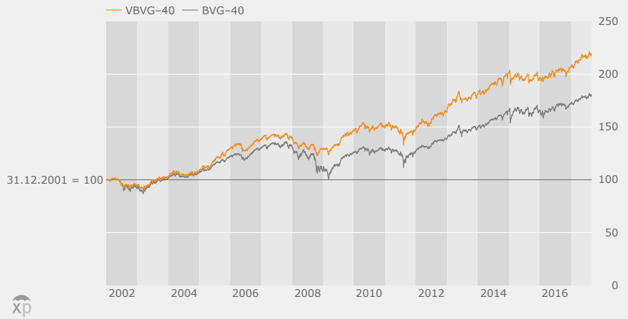
Fundo VBVG-40 vs BVG-40 01.01.02–31.08.17
