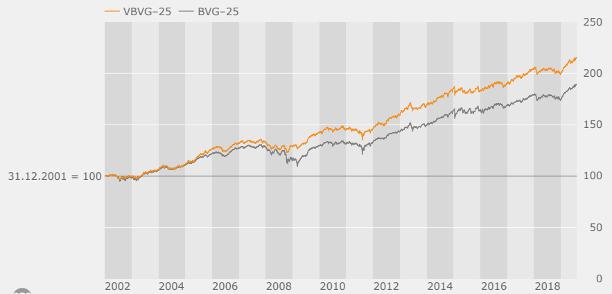
Fundo VBVG-25 vs BVG-25 01.01.02–31.07.19
