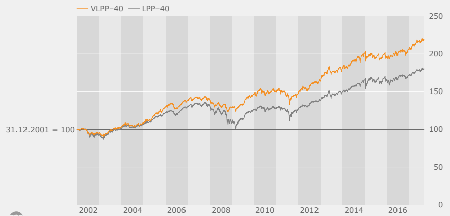
Fundo VLPP-40 vs LPP-40 01.01.02–31.08.17
