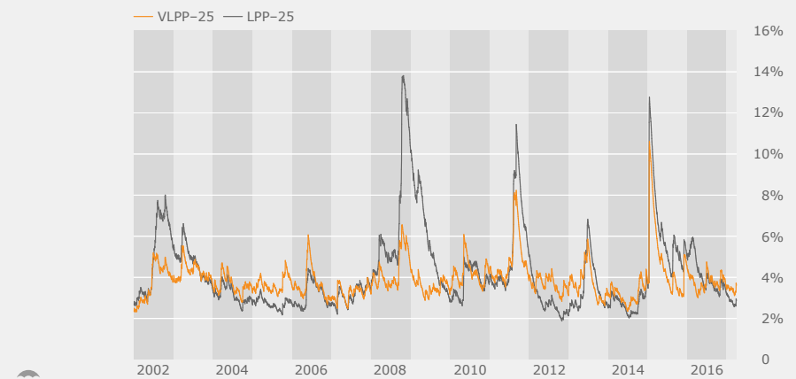
VLPP-25 vs LPP-25 Ex Post Volatility 01.01.02–31.03.17
