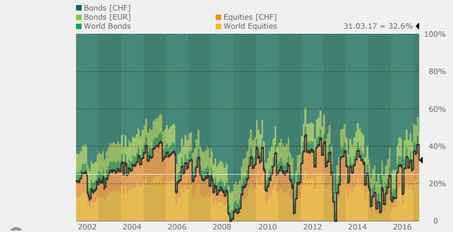
Fundo VLPP-25 Asset Class Weightings 01.01.02–31.03.17
