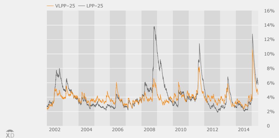
VLPP-25 vs LPP-25 Ex Post Volatility 01.01.02–29.05.15
